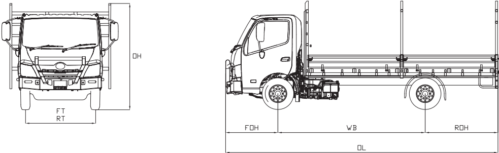
Drawings are for reference only to the dimensions table above. For specific layouts please refer to the applicable Body Mounting Manual (BMM).
